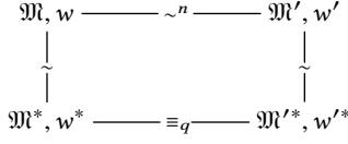
Figure 1: Generic upgrading pattern.
