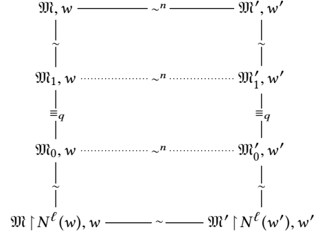
Figure 2: Upgrading pattern for Theorem 2.
